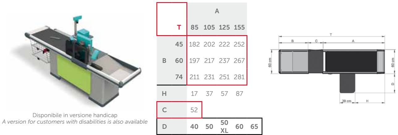
SINGOLO VASCA LARGA - RULLIERA • NARROW SINGLE BASIN - FRONT CABINET - ROLLER TABLE
